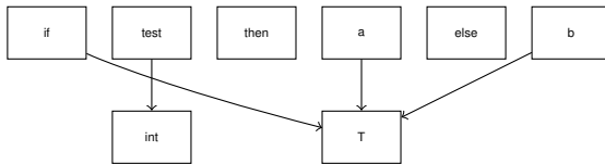
FIGURE 1 – if/then/else
